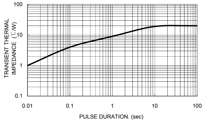
FIG. 6- TYPICAL TRANSIENT THERMAL CHARACTERISTICS
