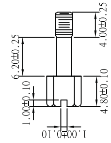
UNC #4-40 Hexscrew
