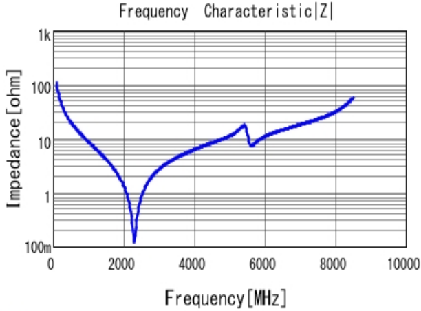
GJM1555C1H150JB01 |Z| DC0V, 25degC
