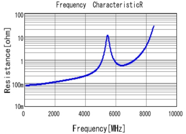
GJM1555C1H150JB01 R DC0V, 25degC
