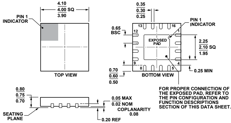
Figure 60. 16-Lead Lead Frame Chip Scale Package [LFCS] 4 mm x 4 mm Body and 0.75 mm Package Height (CP-16-23) Dimensions shown in millimeters
