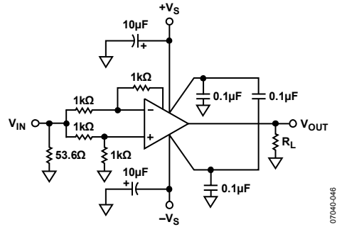
Figure 52. Common-Mode Rejection
