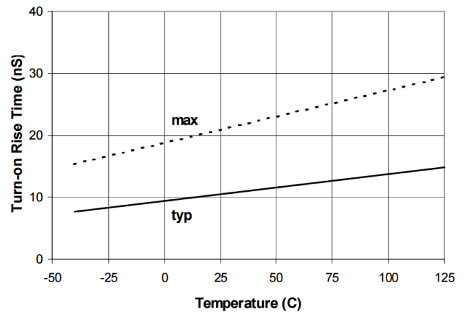
Figure 10A. Turn-on Rise Time vs. Temperature
