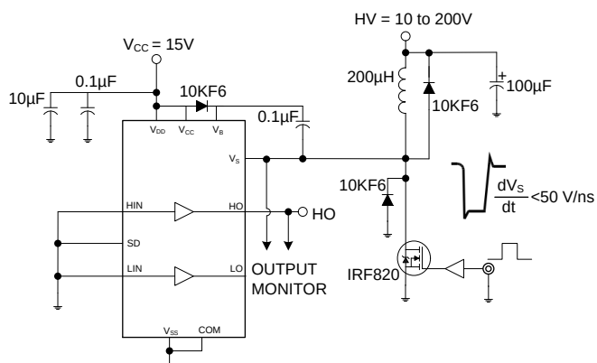
Figure 2. Floating Supply Voltage Transient Test Circuit
