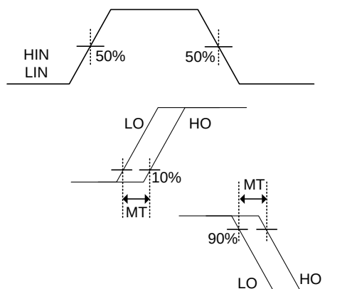
Figure 6. Delay Matching Waveform Definitions
