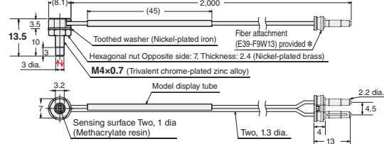
11-E E32-D21N 2M (Free Cutting)
