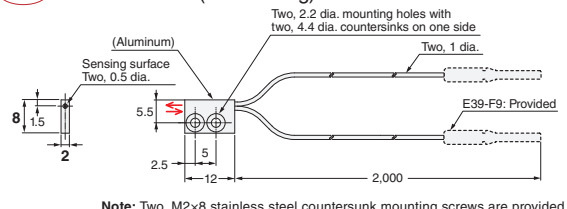
47-F E32-D25XB 2M (Free Cutting)
