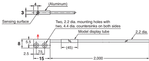
17-C E32-T15YR 2M (Free Cutting)
