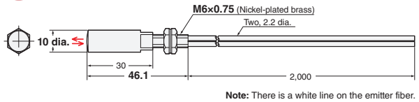
27-H E32-C91N 2M (Free Cutting) + E39-F18
