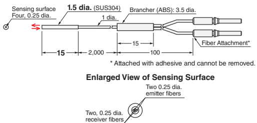
47-A E32-D22B 2M (No Cutting)
