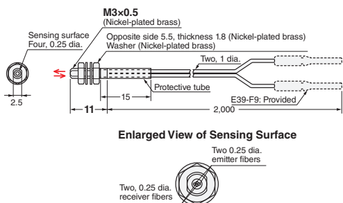
47-B E32-D21 2M (Free Cutting)
