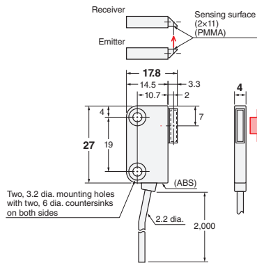
53-B E32-T16JR 2M (Free Cutting)
