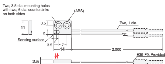
37-B E32-L24S 2M (Free Cutting)
