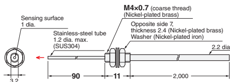
21-E E32-TC200BR 2M (Free Cutting)
