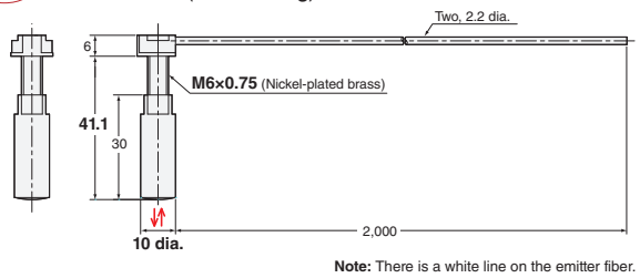
27-H E32-C91N 2M (Free Cutting) + E39-F18
