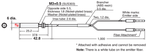
27-E E32-C31 2M (Free Cutting) + E39-F3B
