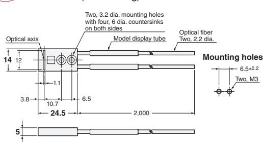
59-D E32-A12 2M (Free Cutting)
