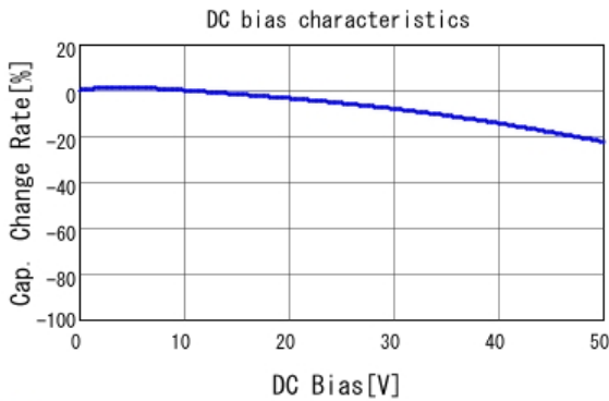
GCM155R71H221KA37 C-DC bias capchange, 25.0degC, AC1.
