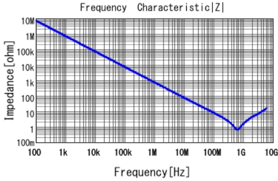
GCM155R71H221KA37 |Z| DCOV, 25degC
