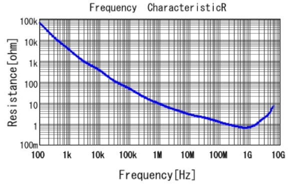
GCM155R71H221KA37 R DCOV, 25degC
