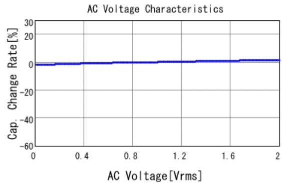
GCM155R71H221KA37 C-AC Voltage capchange, DCOV, 25.0d
