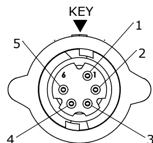
FACE VIEW W16980-5SG-P-5XX 5 POSITION A-KEY
