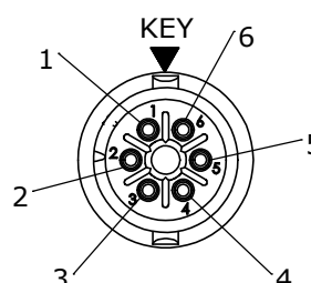
WIRING VIEW W16980-6SG-P-5XX
