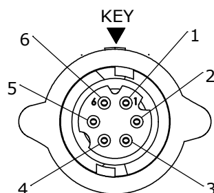
FACE VIEW W16980-6SG-P-5XX 6 POSITION B-KEY
