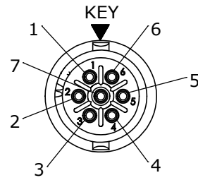
WIRING VIEW W16980-7SG-P-5XX
