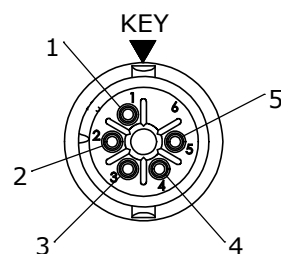
WIRING VIEW W16980-5SG-P-5XX
