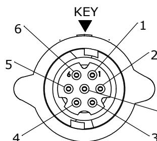
FACE VIEW W16980-7SG-P-5XX 7 POSITION A-KEY
