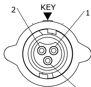
FACE VIEW W16282-3PG-P-3XX
