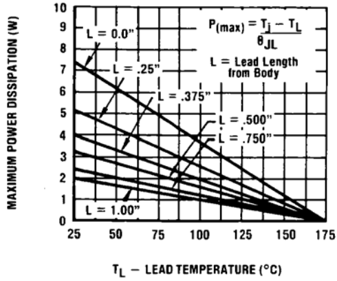
FIGURE 3 MAXIMUM POWER vs LEAD TEMPERATURE
