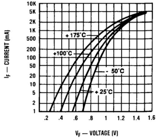
FIGURE 4 TYPICAL FORWARD VOLTAGE vs FORWARD CURRENT
