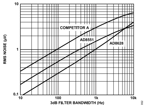
Figure 55. RMS Noise vs. 3 dB Filter Bandwidth in Hz
