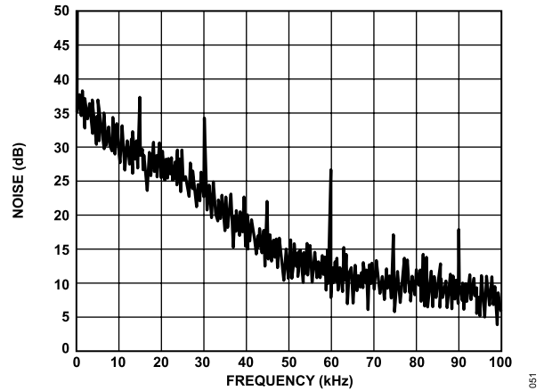
Figure 54. Actual Transfer Function of the Test Circuit in Figure 52
