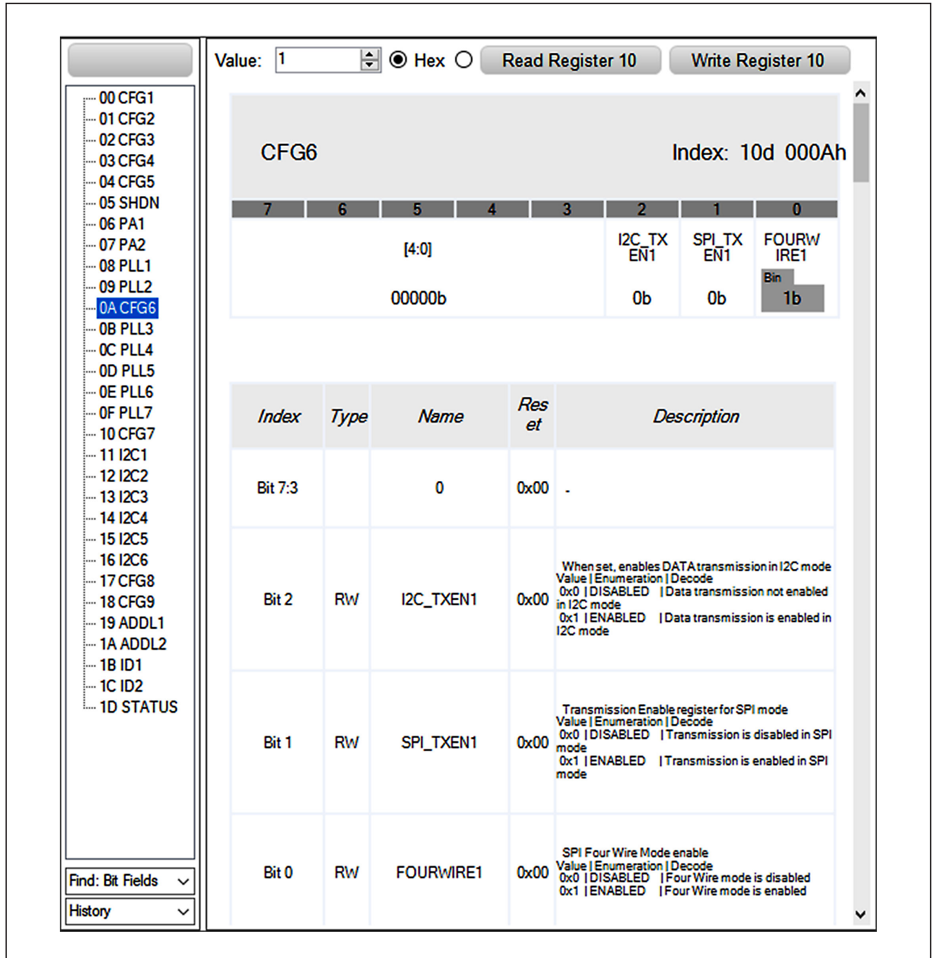
Figure 15. 4-Wire SPI Setting.
