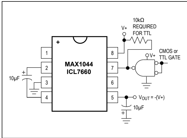
Figure 7. External Clocking
