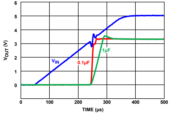
FIGURE 114. TURN-ON TIME
