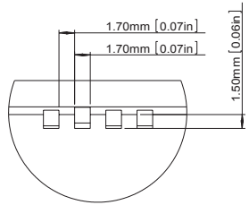
SECTION C SCALE 3:1
