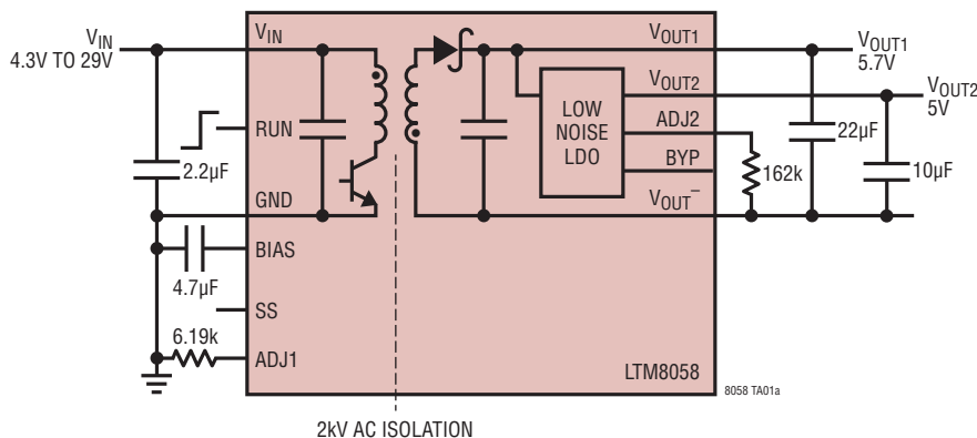
2kV AC Isolated Low Noise \mu Module Regulator
