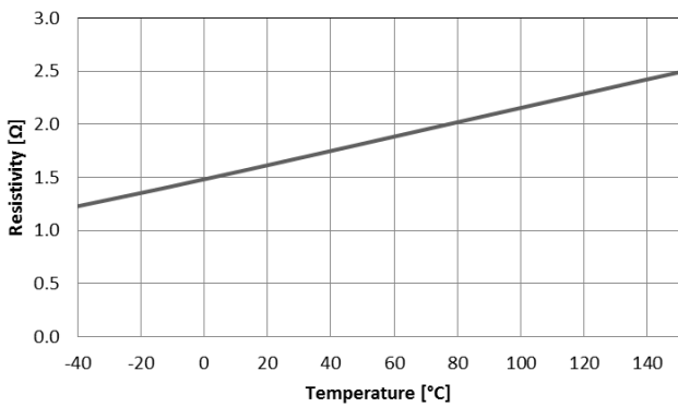
Figure 23. R_{ON} vs. Temperature
