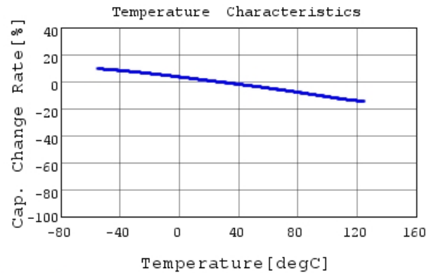
GR442QR73D101KW01 C-Temp. capchange, DCOV, 1
