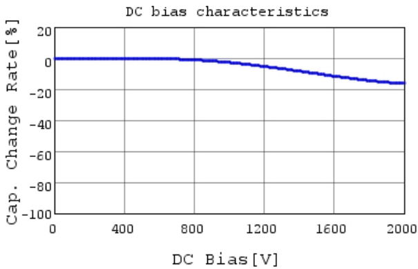
GR442QR73D101KW01 C-DC bias capchange, 25.0c
