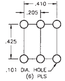
Mounting Detail
