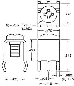
Mounting Detail
