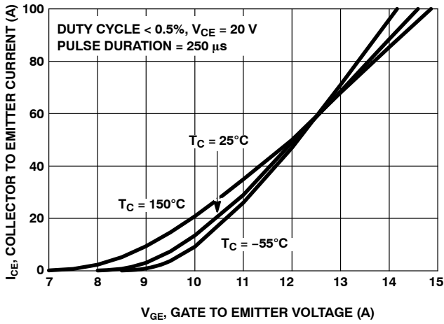
Figure 13. TRANSFER CHARACTERISTIC
