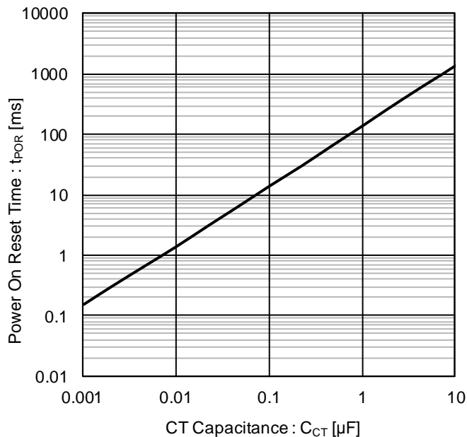
Figure 19. Power on Reset Time vs CT Capacitance
