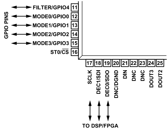
Figure 114. AD7768-4 GPIO Functionality
