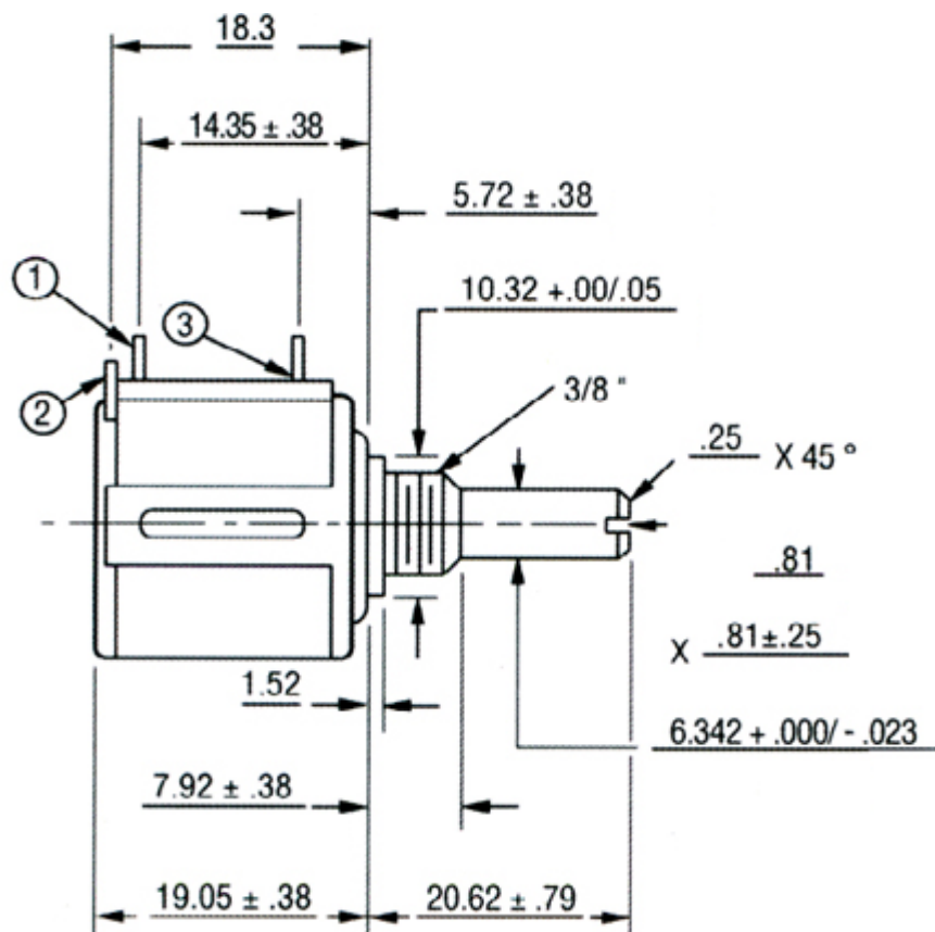
3590S-2 100 Ohm
