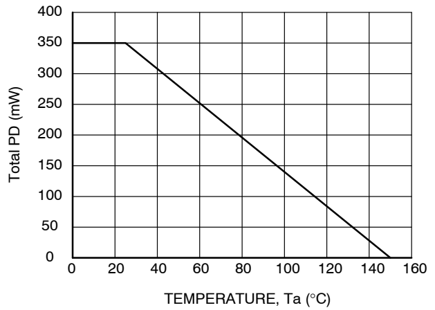
Figure 10. Total PD vs. Temperature
