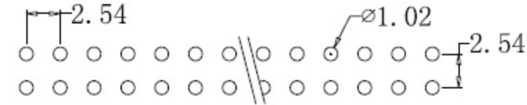
PCB LAYOUT
