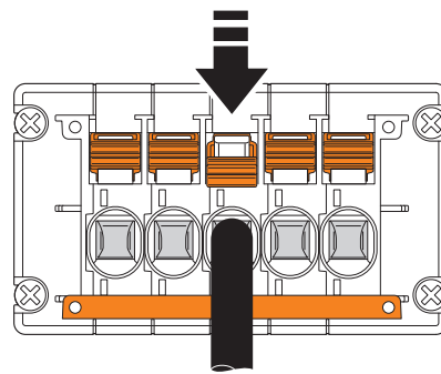
Figure 17 Inserting the conductor
