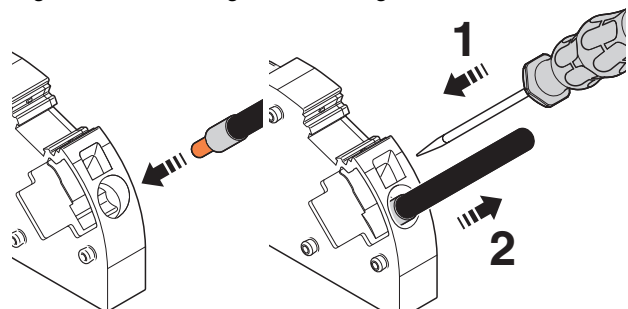
Figure 15 Inserting and releasing the conductor
