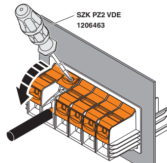
Figure 21 Closing the terminal point
