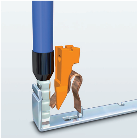
Figure 13 Push-in connection
