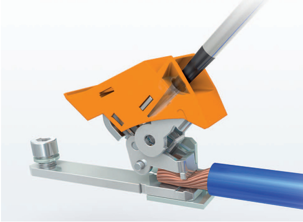
Figure 19 T-LOX
