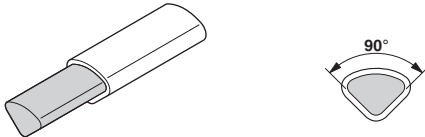
Figure 26 Structure of sector-shaped conductors
