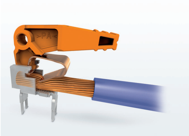
Figure 16 Push-Lock connection
