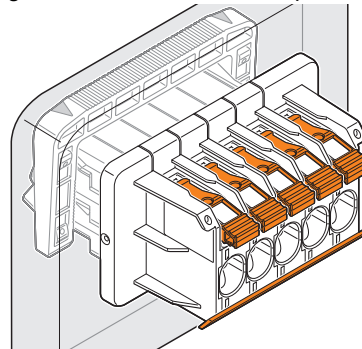
Figure 18 Closed terminal point
