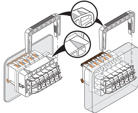
Figure 10 Placing the spacer adapter (DP) and the terminal wedge
