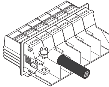
Figure 23 Inserting the conductor (example shows TW...-CL...)
