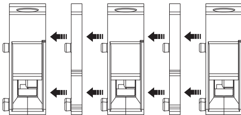
Figure 6 Spacer plates (terminals shown are examples)
