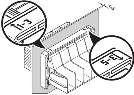
Figure 8 Orientation in which to place the wedge
