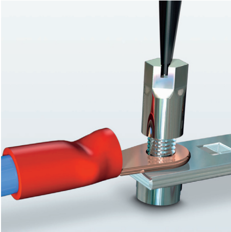
Figure 22 Bolt connection
