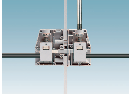
Figure 12 Connecting a conductor to an HDFK terminal
