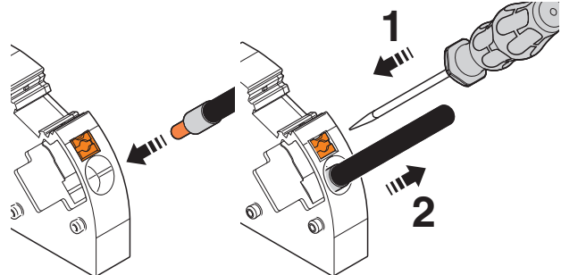
Figure 14 Inserting and releasing the conductor
