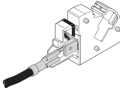
Figure 25 Connecting the conductor (PW...-POT-SCM...)
