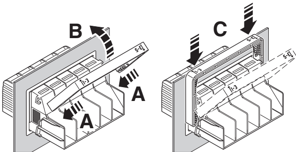
Figure 9 Placing the wedge
