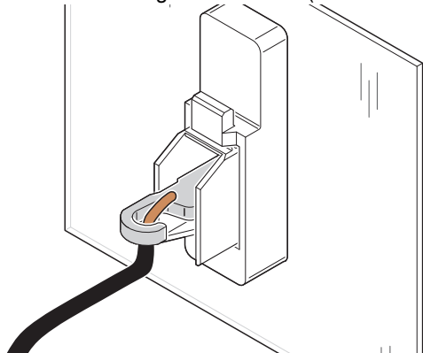
Figure 24 Connecting the conductor (PW...-POT-SL...)
