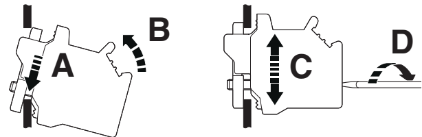
Figure 7 Mounting the DFK 4-PE
