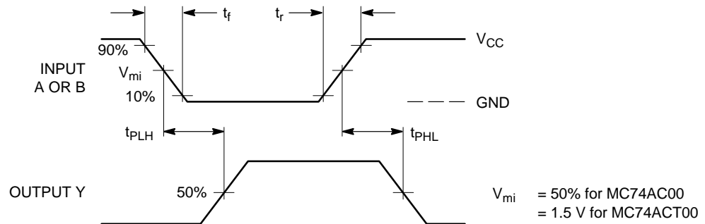
Figure 3. Switching Waveforms
