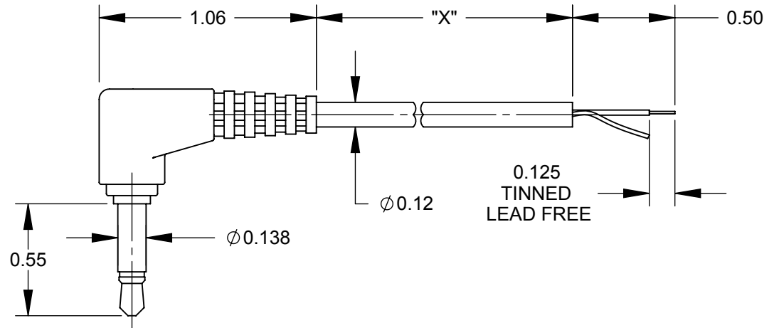
3.5MM MONO PLUG
