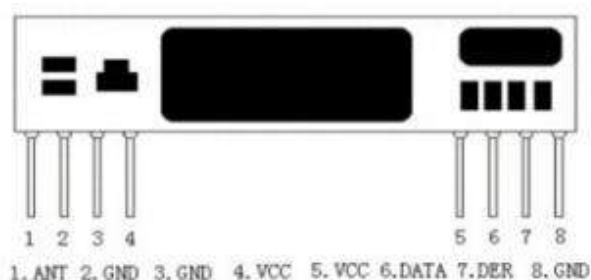
Figure1 CY71 Shape & Pins
