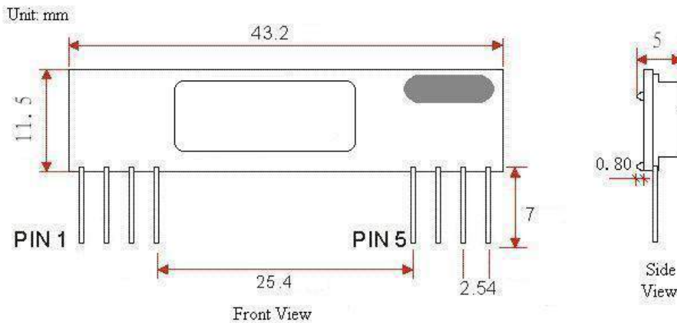
Figure2 CY71 Dimension
