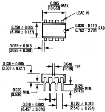
8 Lead Plastic DIP \theta_{JA} = 120^{\circ}\text{C/W} \theta_{JC} = 70^{\circ}\text{C/W}
