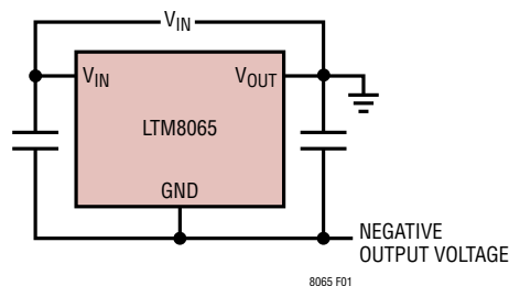
Figure 1. The LTM8065 Can Be Used to Generate a Negative Voltage
