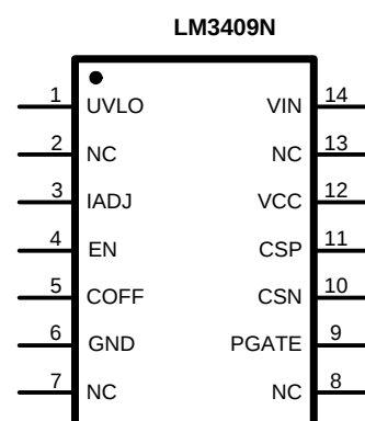
Figure 2. 14-Lead PDIP Package
