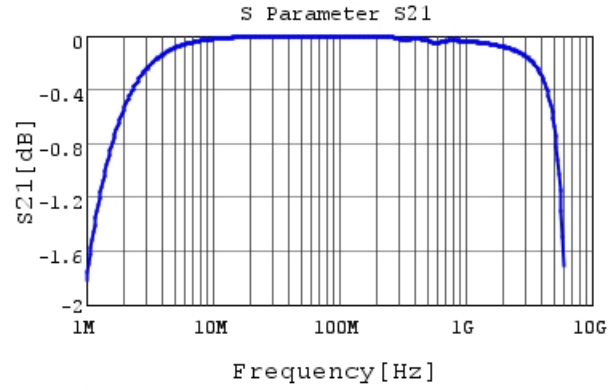
GRM3195C2A222JA01 S21 DCOV, 25degC
