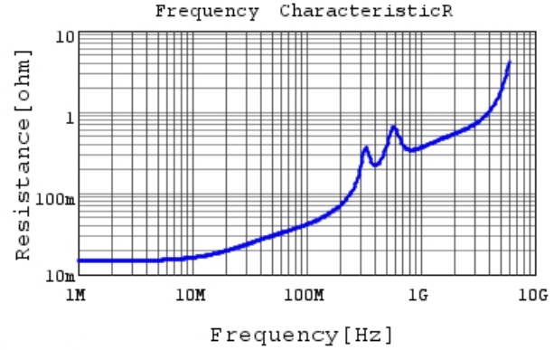
GRM3195C2A222JA01 R DCOV, 25degC
