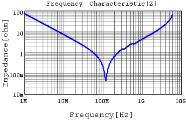
GRM3195C2A222JA01 |Z| DCOV, 25degC
