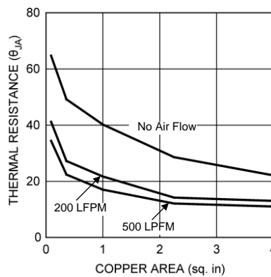
Figure 36. Thermal Resistance vs PCB Area
