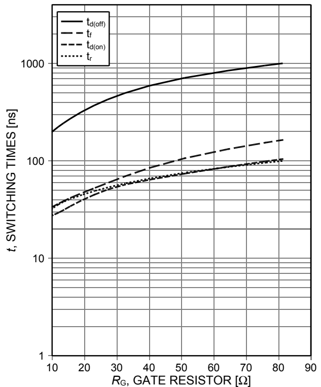
Figure 8. Typical switching times as a function of gate resistor (ind. load, T_j=150^\circ\text{C} , V_{CE}=400\text{V} , V_{GE}=0/15\text{V} , I_c=60\text{A} , test circuit in Fig. E)
