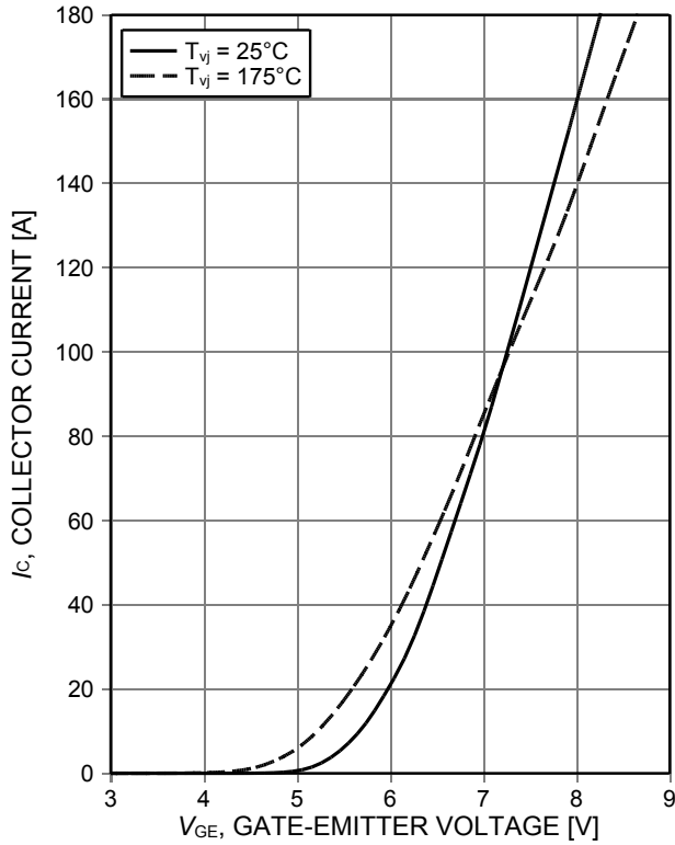
Figure 5. Typical transfer characteristic ( V_{CE}=20\text{V} )
