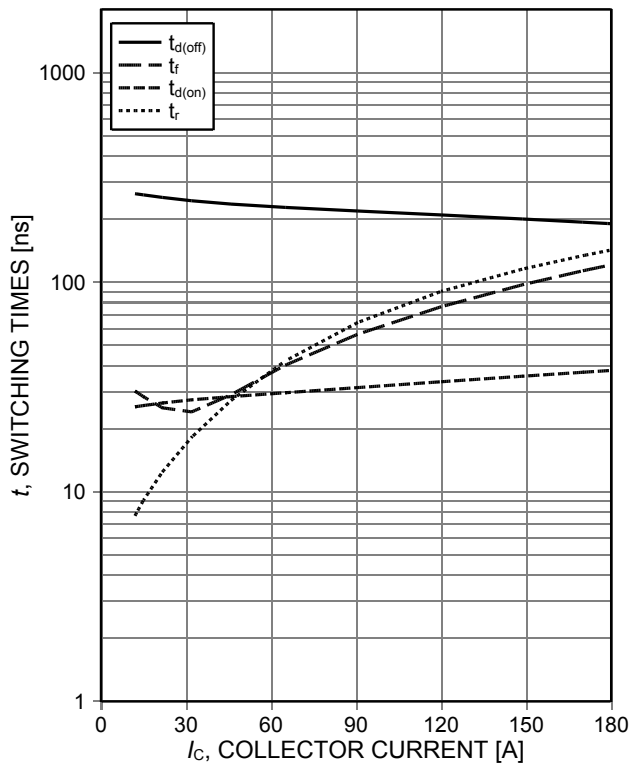
Figure 7. Typical switching times as a function of collector current (ind. load, T_j=150^\circ\text{C} , V_{CE}=400\text{V} , V_{GE}=0/15\text{V} , R_G=12\Omega , test circuit in Fig. E)
