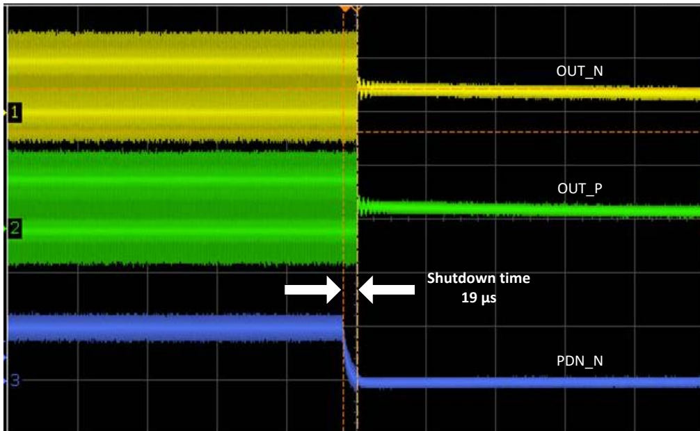
Figure 16: Shutdown timing (19 \mu s from de-asserting PDN_N to zero output)
