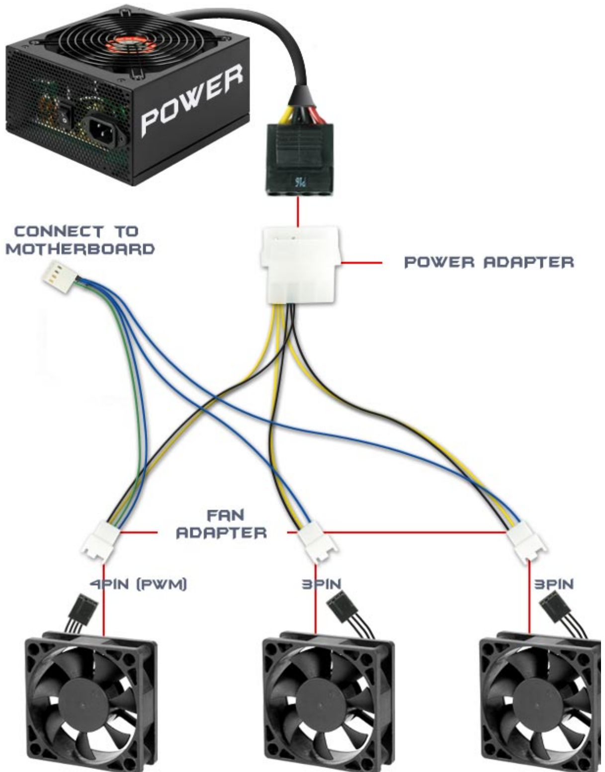
Cable Schematic
