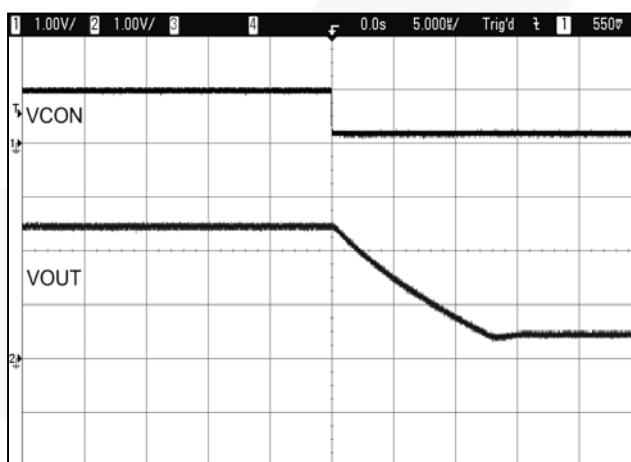
Figure 39. V_{OUT} Falling Transition 3.0 V to 0.5 V, V_{IN} = 3.7\text{ V} in High-Power Mode
