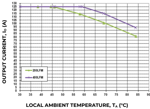
Figure 17. Output Current Derating for the Base plate QBDS125A10R4-H+0.6" Heat Sink; Airflow Direction for Vout to Vin (Worst) orientation; Vin = 50V.
