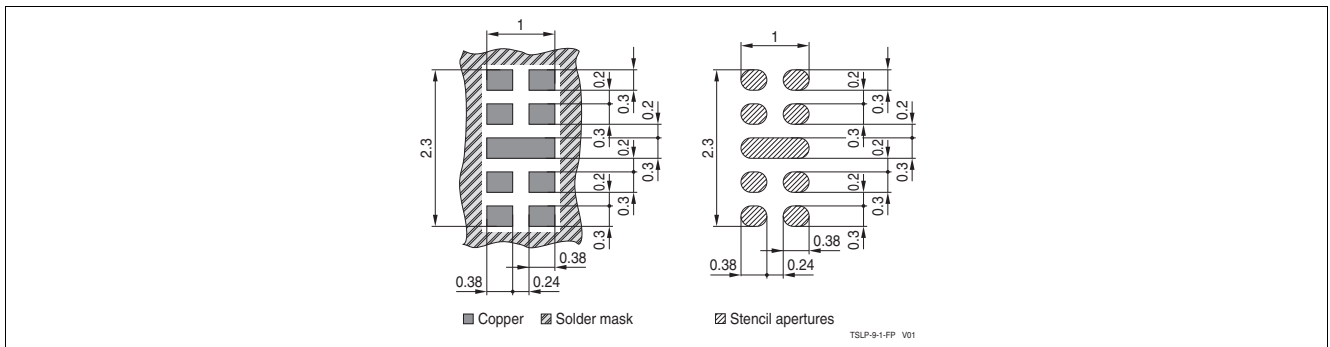
Figure 15 TSLP-9-1: Footprint
