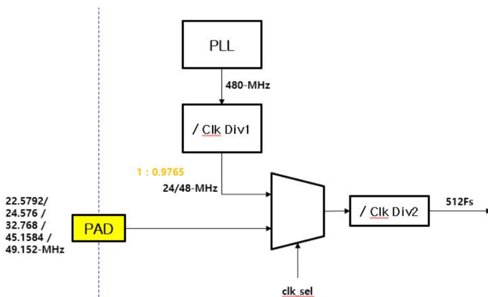
Figure 25: I2S Clock Scheme
