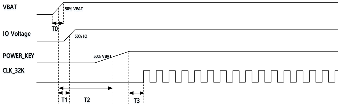
Figure 7: Power on Sequence
