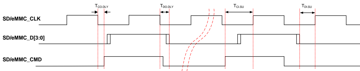
Figure 23: SD/eMMC Master Timing Diagram
