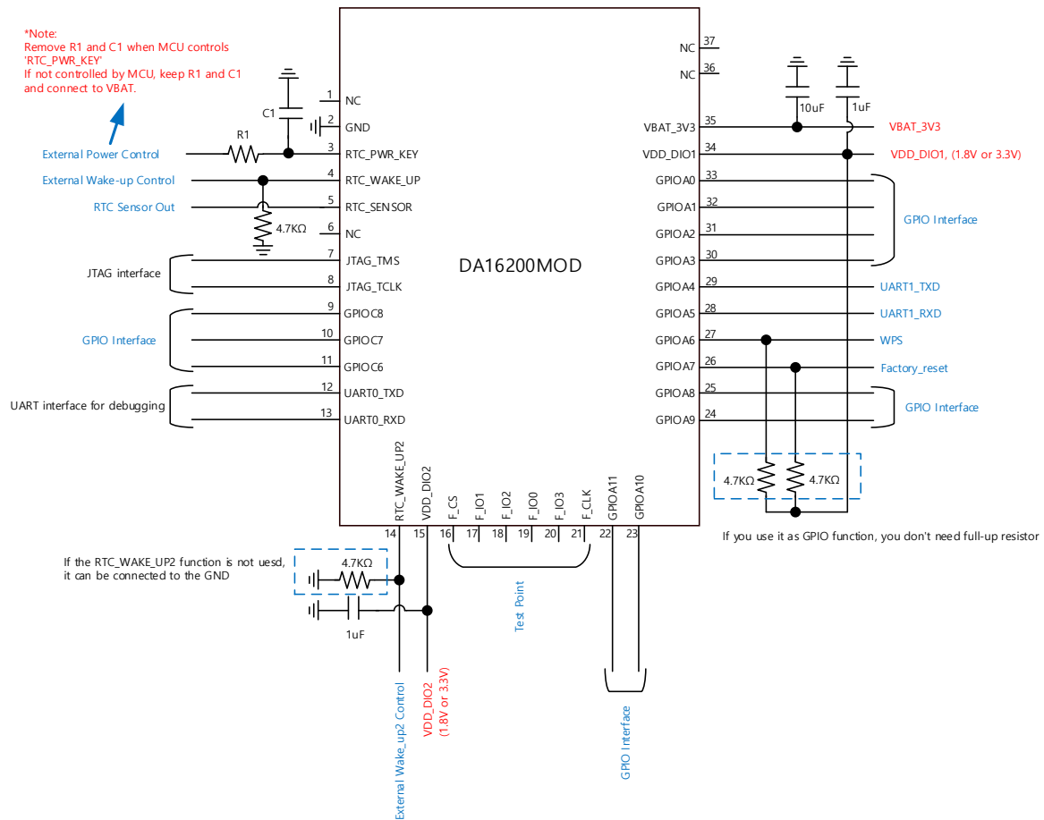
Figure 44: Application Schematic
