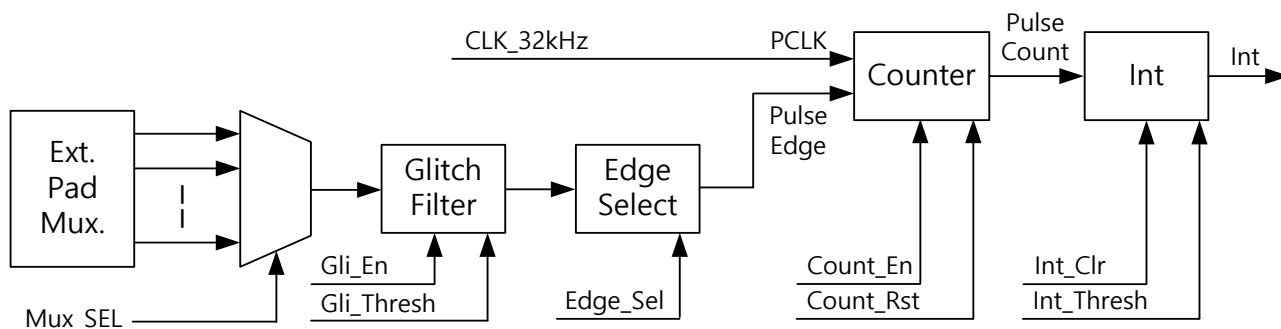
Figure 8: Pulse Counter Block Diagram
