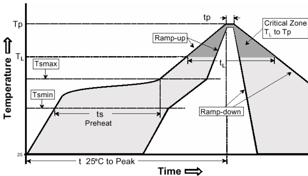
Figure 51: Reflow Condition
