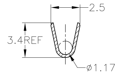
SECT. C-C
