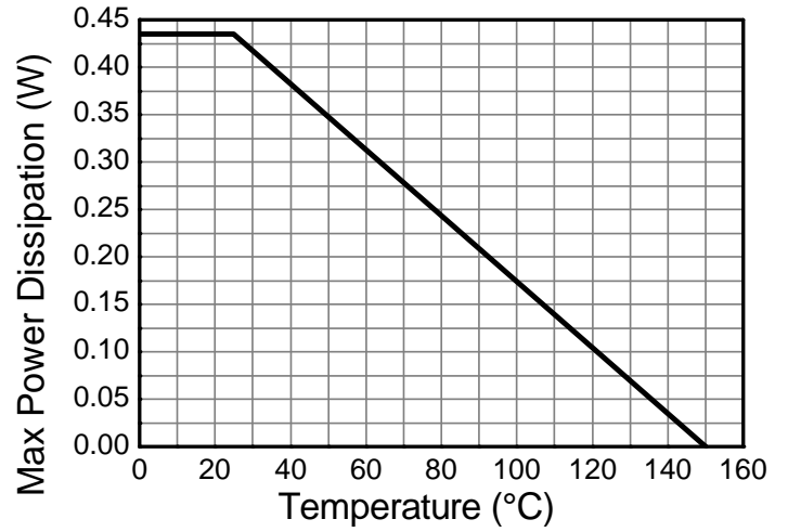
Derating Curve
