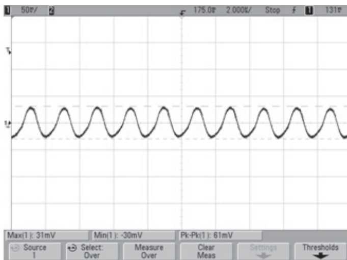
Output ripple and Noise (V in =48V, I out =0, Cload= 1uF || 10uF, T a =+25°C) Vout ripple=61mV
