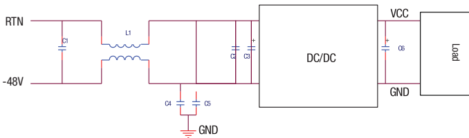
Figure 4. Conducted Emissions Test Circuit
