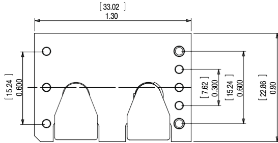
PIN SIDE VIEW
