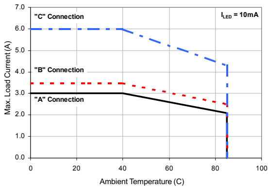
Figure 1. Typical Current Derating Curves*
