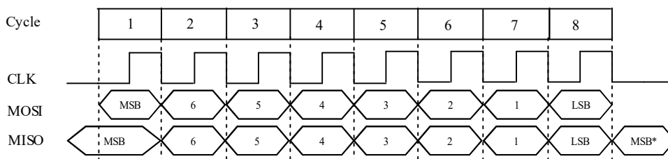
Figure 10-1 模式0时序图 Transport Format of SPI Mode 0
