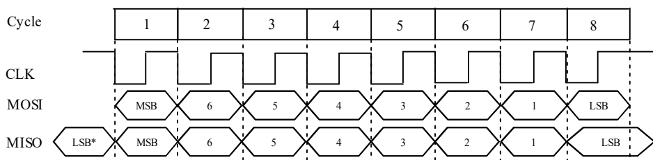
Figure 10-2 模式3时序图 Transport Format of SPI Mode 3
