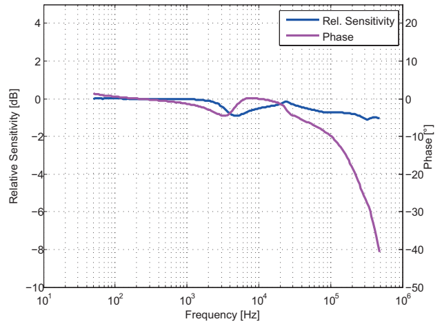
Figure 2: Frequency response
