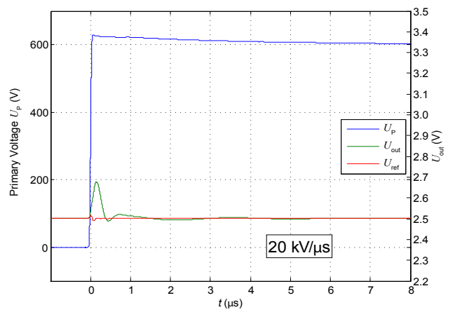
Figure 10: du/dt
