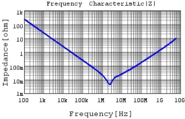
GRM188R60J106ME47 |Z| DCOV, 25degC
