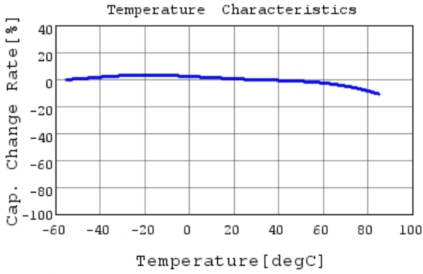
GRM188R60J106ME47 C-Temp. capchange, DC0.0V,
