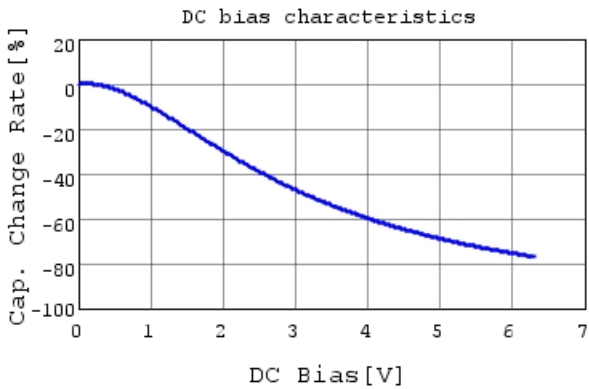
GRM188R60J106ME47 C-DC bias capchange, 25.0c
