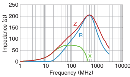
KMZ1608YHR102BTD25
