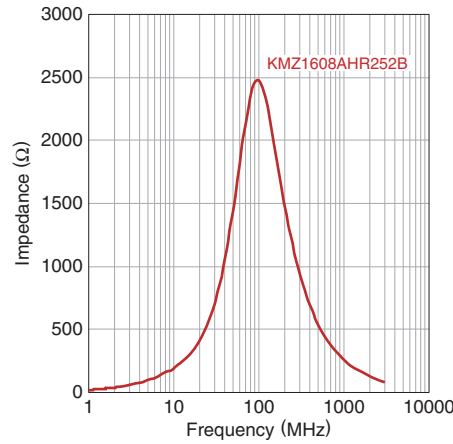
KMZ1608AHR series
