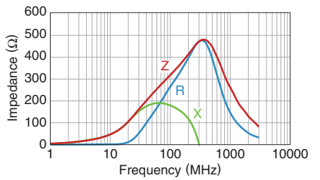
KMZ1608YHR152BTD25
