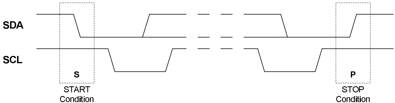
Figure 20-3. START and STOP Conditions
